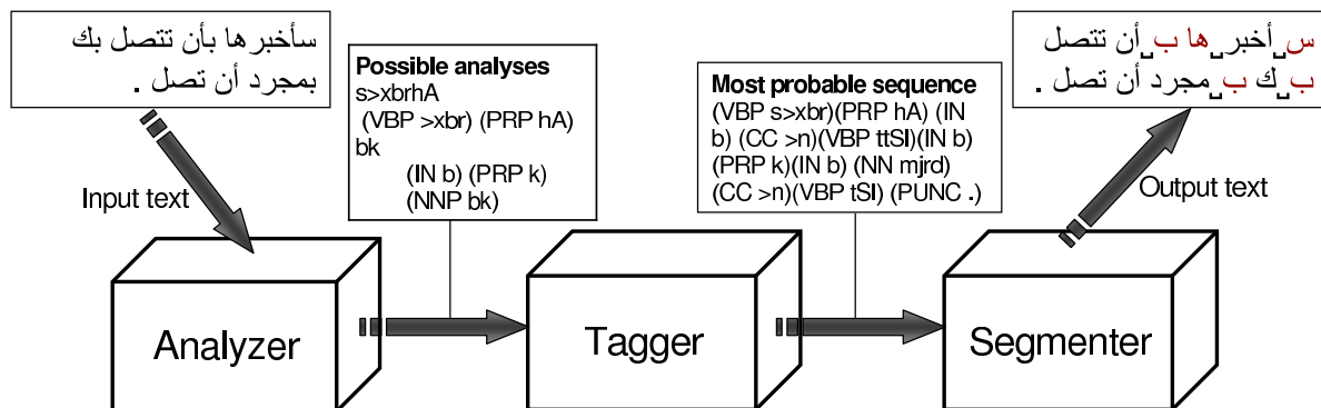
Figure 2: MorphTagger segmenter architecture
