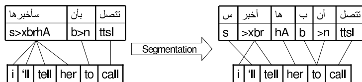
Figure 1: Arabic segmentation example: Arabic words are accompanied by the Buckwalter transliteration and the alignment to the words on the English side
