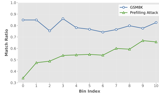
Figure 3: Mean match ratio of utility and safety tasks.
