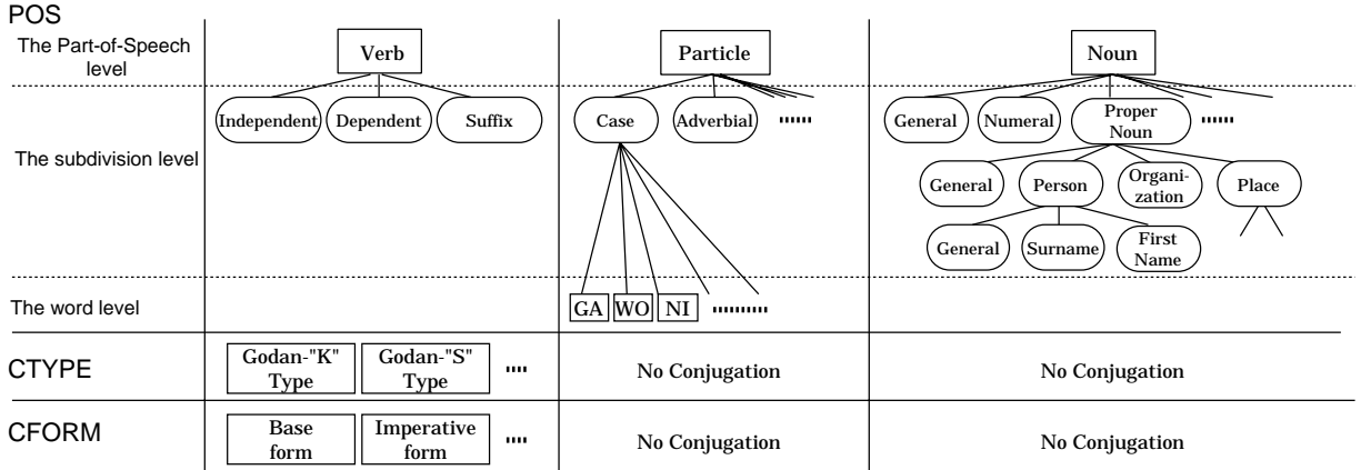
Figure 1: The examples of the hierarchical tag set
