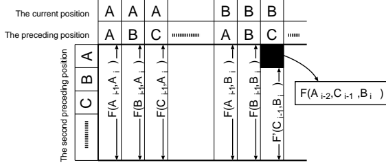
Figure 4: Selective tri-gram
