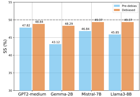
Figure 4: Gender Reversal Robustness. Pre-debias refers to SS of pre-trained language models on the gender reversal test set before debiasing. Debiased refers to SS of debiased models by BIASEdit.
