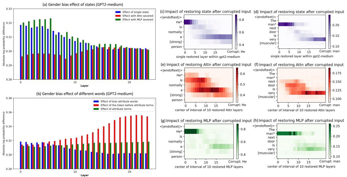
Figure 5: Gender bias tracing on GPT2-medium. (a) Comparing bias associations of bias attribute words on hidden states, attention layers, and MLP layers. (b) Comparing bias associations on single states of the bias attribute word, the token before the attribute term, and the attribute term. The bias impacts on output probability are mapped for the effect of (c-d) each hidden state on the context, (e-f) only MLP activations, and (g-h) only attention activations. * marks the corrupted bias attribute words and [] refers to the attribute terms in (c-h).
