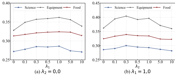
Figure 5: The MRR results of TaxoPro on validation sets, utilizing different auxiliary loss function weight hyperparameters: \lambda_1 for \mathcal{L}_{\text{push}} and \lambda_2 for \mathcal{L}_{\text{pull}} .
