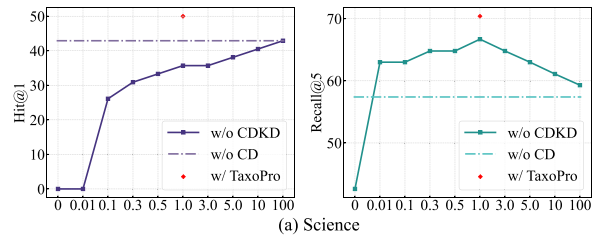
Figure 4: The results of vanilla LoRA-tuned TacoPrompt+Joint (TacoPrompt+TaxoPro w/o CDKD) using different domain loss balance hyperparameter \alpha . Please refer to Appendix A.5 for results on all datasets.
