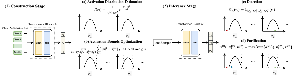
Figure 2: Illustration of our BadActs framework. (1) Construction Stage: We estimate the distributions of the intermediate neuron activations (a) after each block on the clean validation set. Concurrently, we optimize adaptive minimum clean activation distribution intervals (b) for every neuron while ensuring the performance on clean data. (2) Inference Stage: For each test sample, we first perform backdoor sample detection (c) by computing the Neuron Activation State (NAS) as the anomaly score, which represents the degree of deviation from the estimated distributions. Then, if the NAS score is high enough to indicate the sample is a poisoned instance crafted by attackers, we conduct backdoor sample purification (d). Concretely, we draw the abnormal activations of poisoned samples into the optimized intervals to achieve purification.
