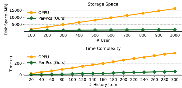
Figure 7: Comparison of storage and time complexity between our PER-PCS and OPPU, demonstrating that PER-PCS requires significantly less time to assemble personal PEFTs and less storage space to save them.
