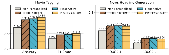
Figure 4: Performance of PER-PCS on movie tagging and news headline generation tasks with different sharer selection strategies. We find PER-PCS is robust to the choice of sharers.
