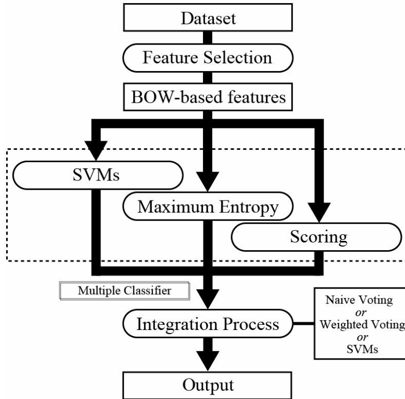
Figure. 1. The outline of our method.
