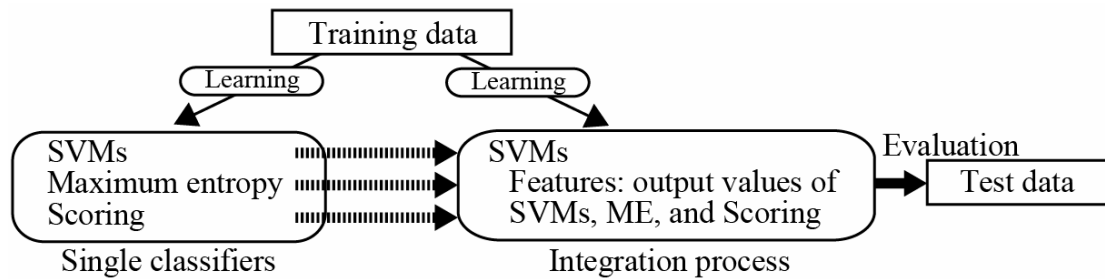
Figure. 2. The integration process with SVMs.
