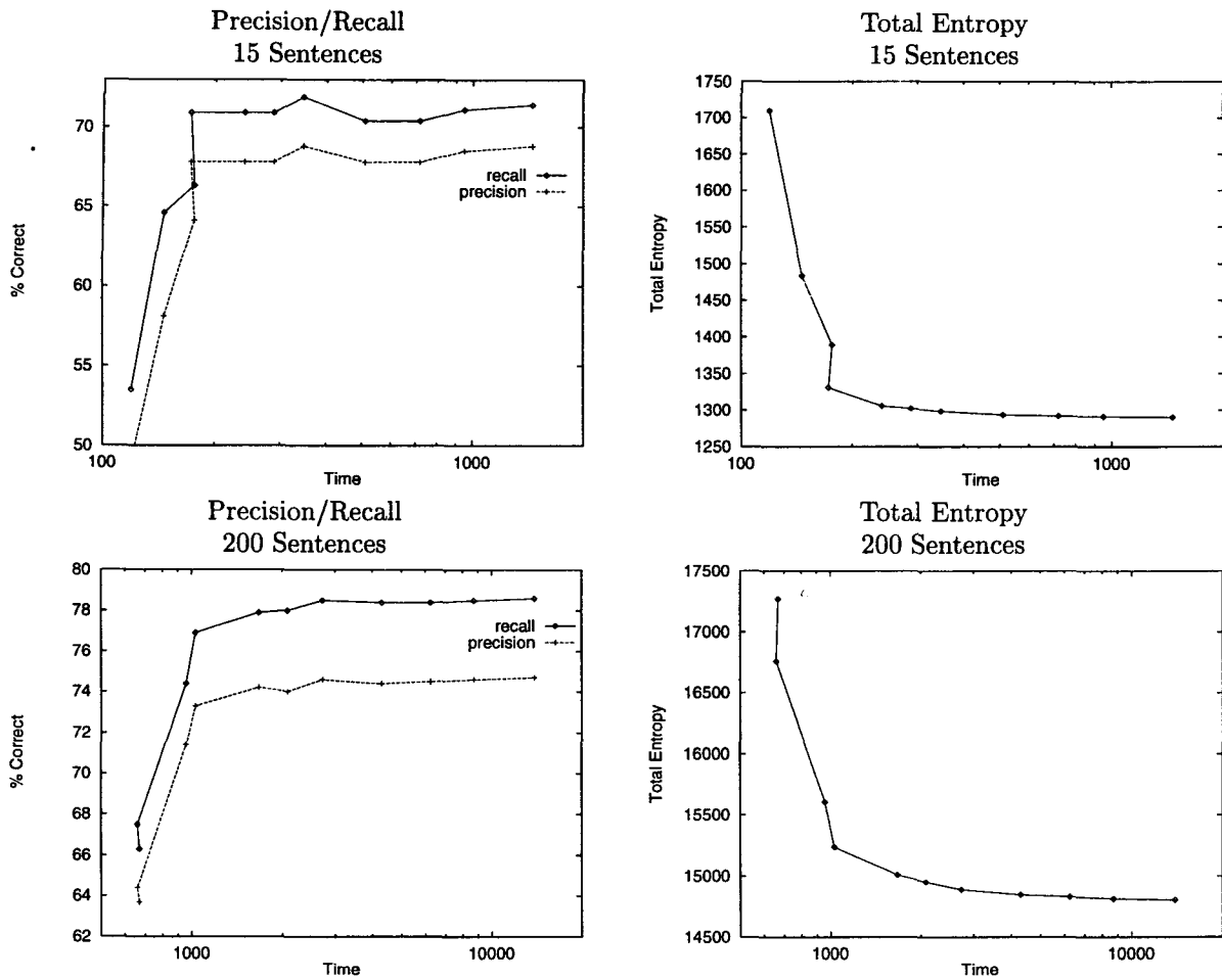
Figure 11: Smoothness for Precision and Recall versus Total Inside for Different Test Data Sizes
