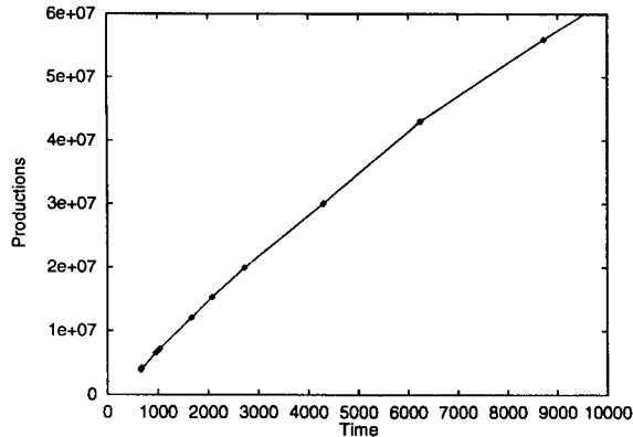
Figure 10: Productions versus Time
