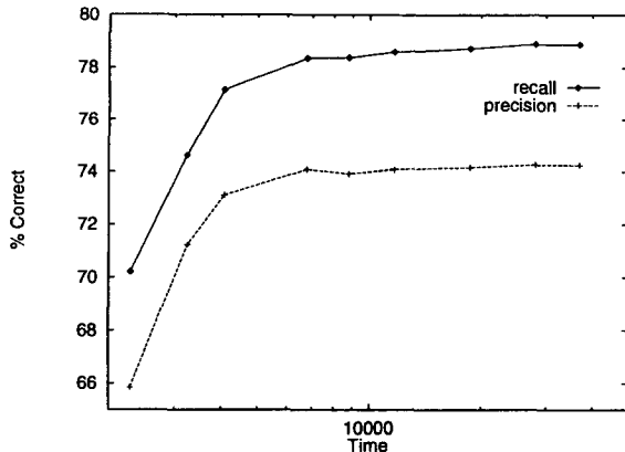
Figure 1: Precision and Recall versus Time in Beam Thresholding
