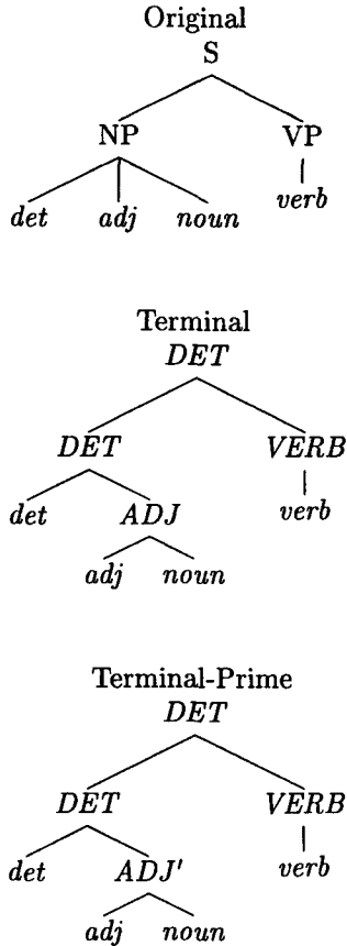
Figure 9: Converting to Terminal and Terminal-Prime Grammars
