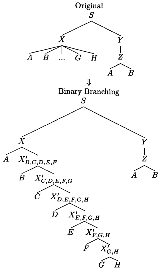
Figure 8: Converting to Binary Branching
