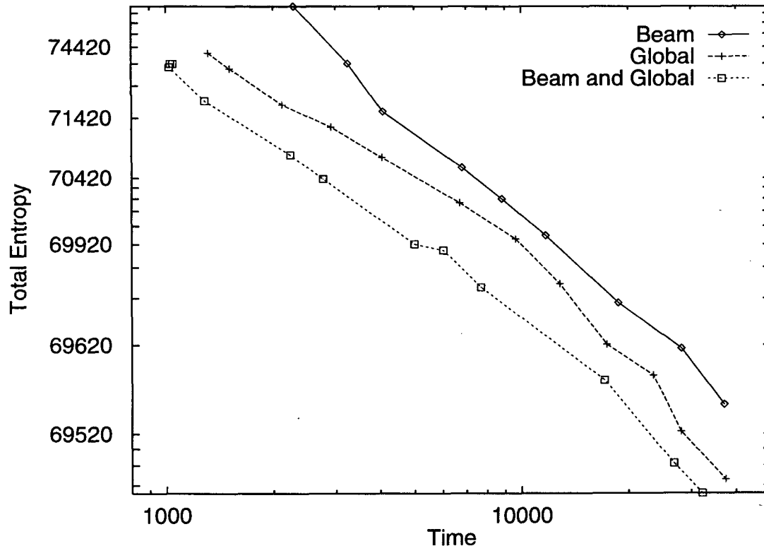
Figure 13: Combining Beam and Global Search
