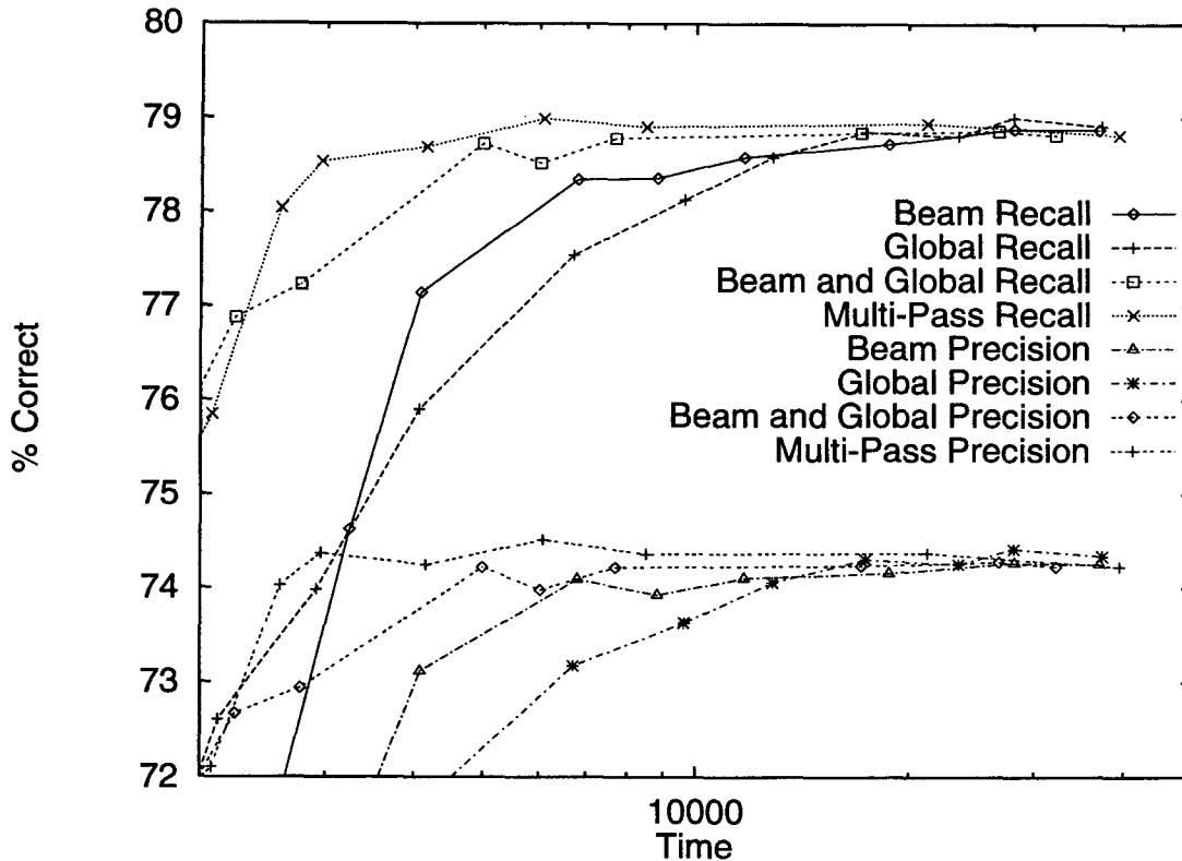
Figure 14: Multiple Pass Parsing vs. Beam and Global vs. Beam
