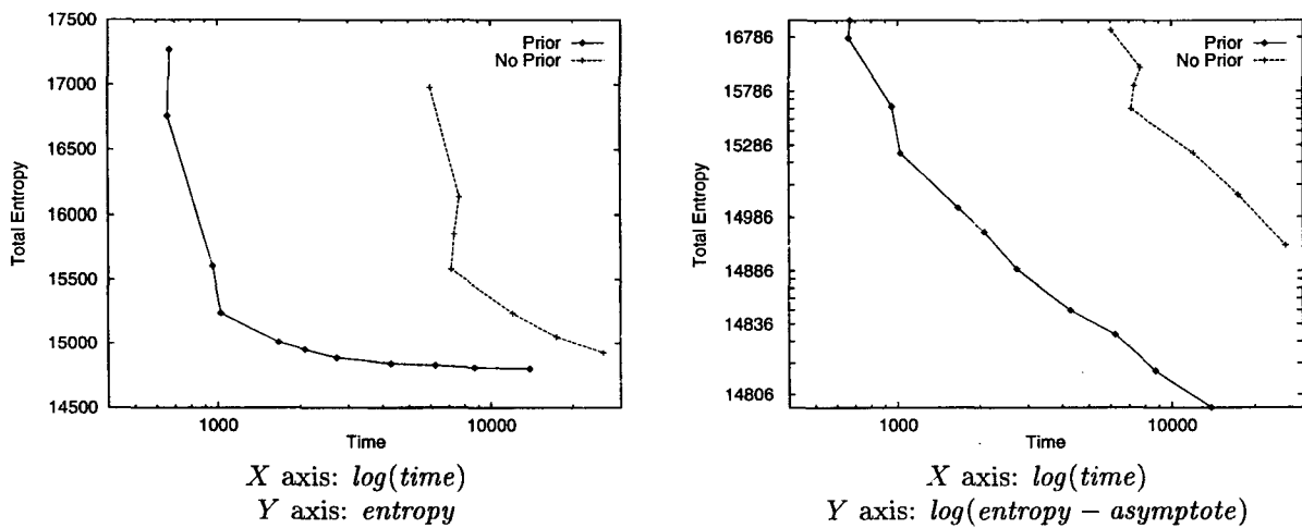
Figure 12: Beam Thresholding with and without the Prior Probability, Two Different Scales
