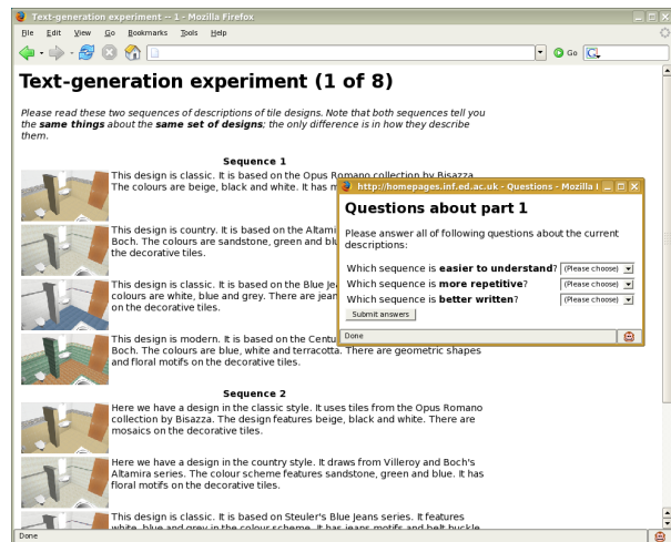
Figure 2: Evaluation interface
