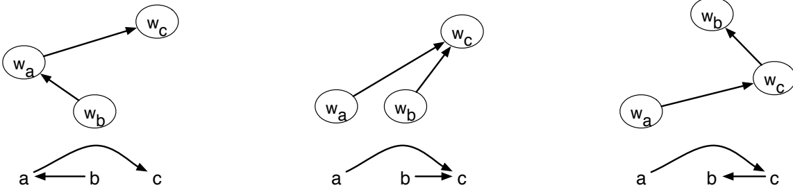
Figure 1: Examples of projective and non-projective trees. The trees on the left and center are both projective. The tree on the right is non-projective.
