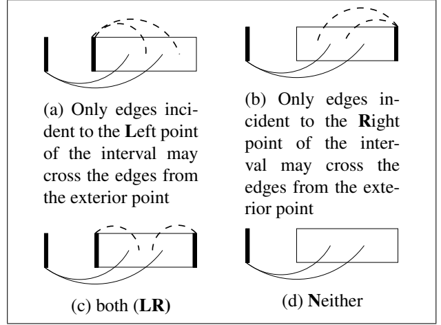
Figure 3: Isolated crossing region sub-problems.
