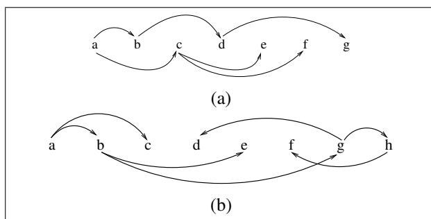
Figure 1: 1a is 1-Endpoint-Crossing, but is neither block degree 2 nor well-nested; 1b is gap-minding but not 2-planar.
