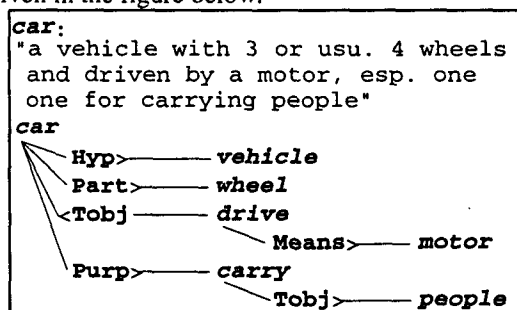
Figure 1. Semrel structure for a definition of car .
