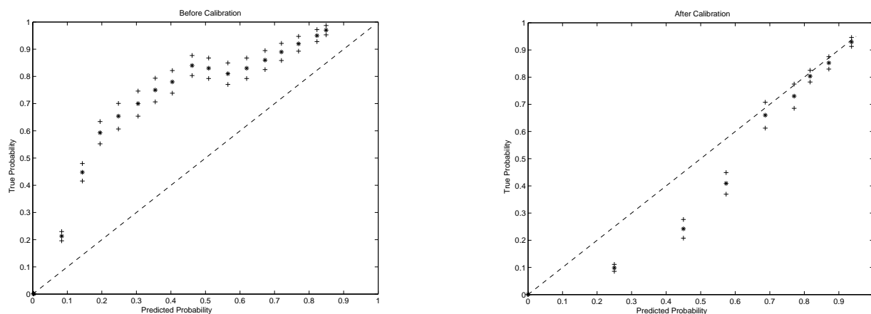
Figure 2: Plots showing true probabilities versus predicted probabilities before and after calibration on the test set for ARGM-TMP.
