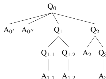
Figure 1: QUD tree
