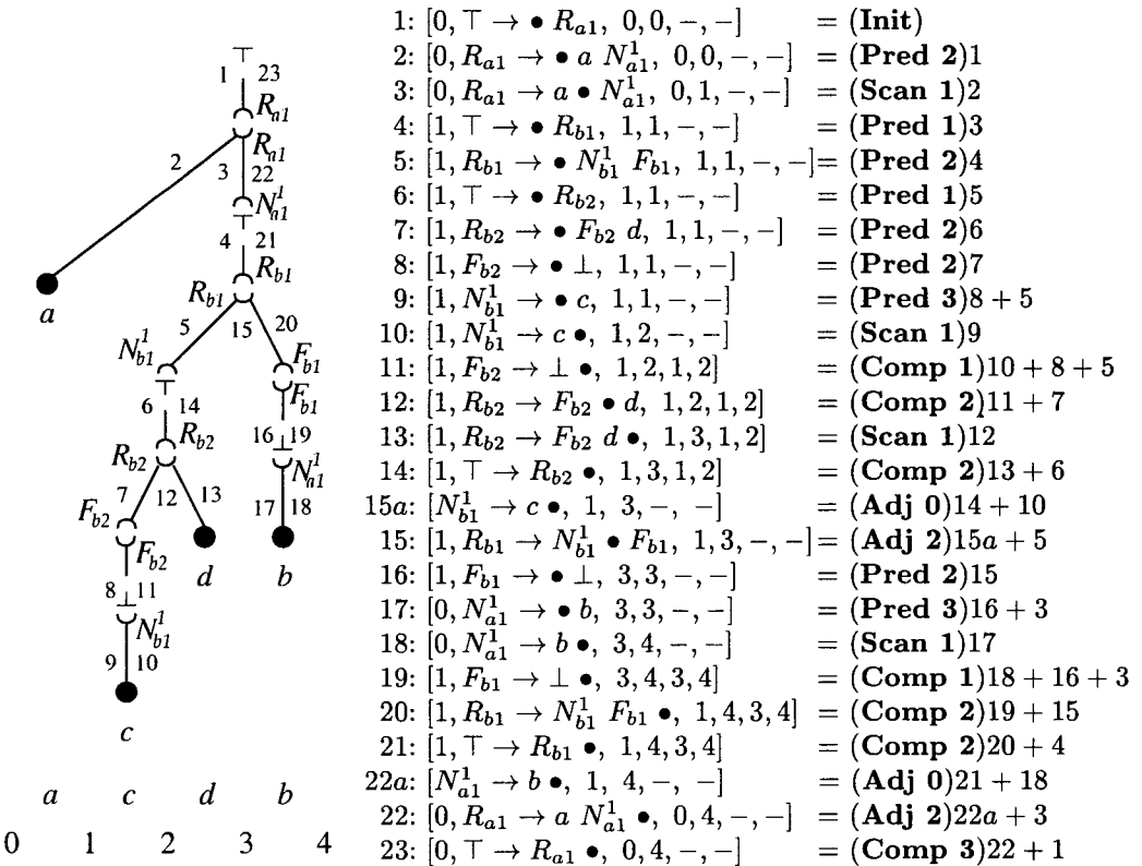
Figure 4 The items needed for recognition of a derived tree.
