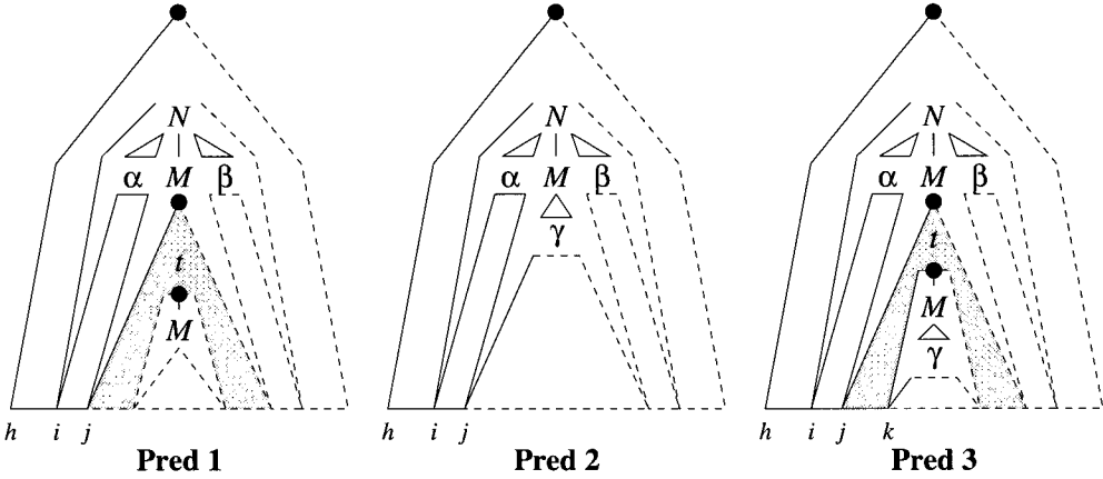
Figure 7 The three predictor steps.
