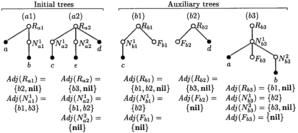
Figure 1 A tree-adjointing grammar.
