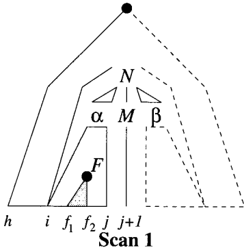
Figure 6 The first scanner step.
