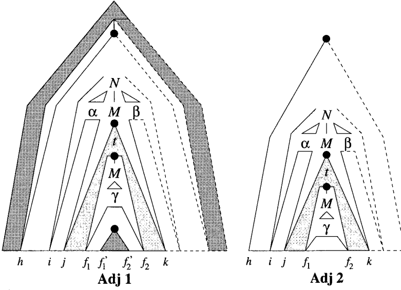
Figure 9 The two adjunction steps, implicitly combined with Adj 0 .
