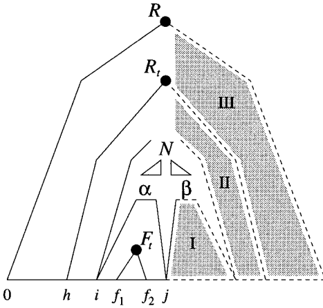
Figure 3 An item [h, N \rightarrow \alpha \bullet \beta, i, j, f_1, f_2] .
