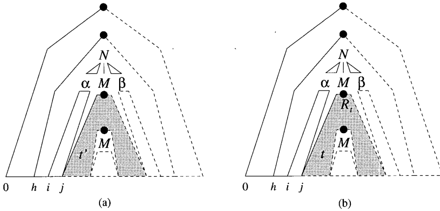
Figure 11 Pred 1 preserves the invariant.
