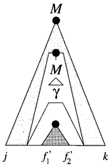
Figure 10 An item [M \rightarrow \gamma \bullet, j, k, f_1', f_2'] .
