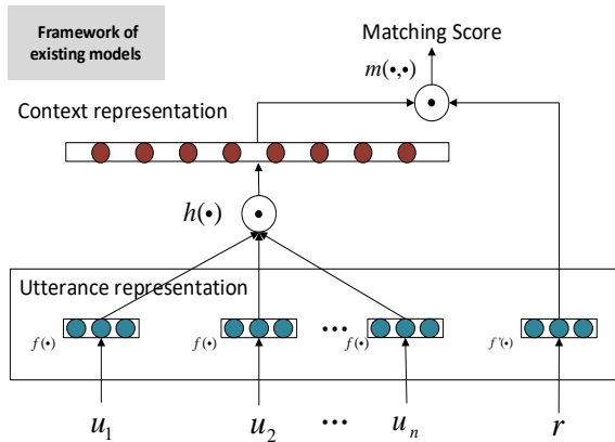
Figure 1 Existing models can be interpreted with a unified framework. f(\cdot), f'(\cdot), h(\cdot) , and m(\cdot, \cdot) are utterance representation function, response representation function, context representation function, and matching function, respectively.
