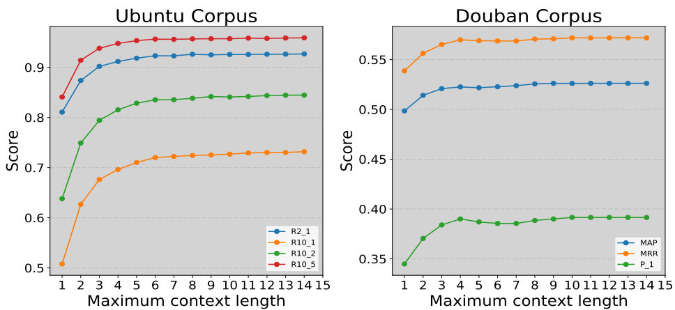
(a) Performance of SCN across different context lengths.
