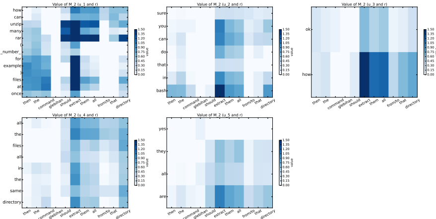
(b) Visualization of M_2 in SCN. Darker squares refer to higher values.
