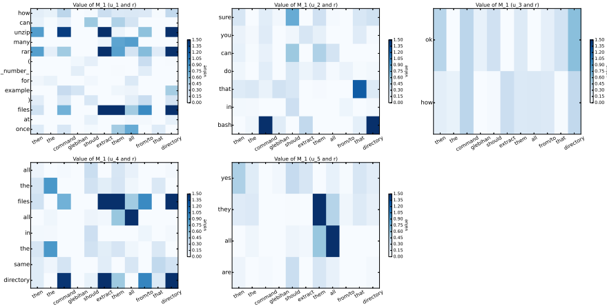
(a) Visualization of M_1 in SCN. Darker squares refer to higher values.
