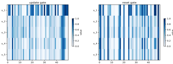
(c) Visualization of gates. Darker squares refer to higher values.
