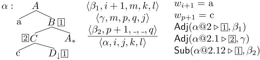
Figure 9 The deductive rule generated for tree \alpha using the baseline TL-MCTAG parsing method.
