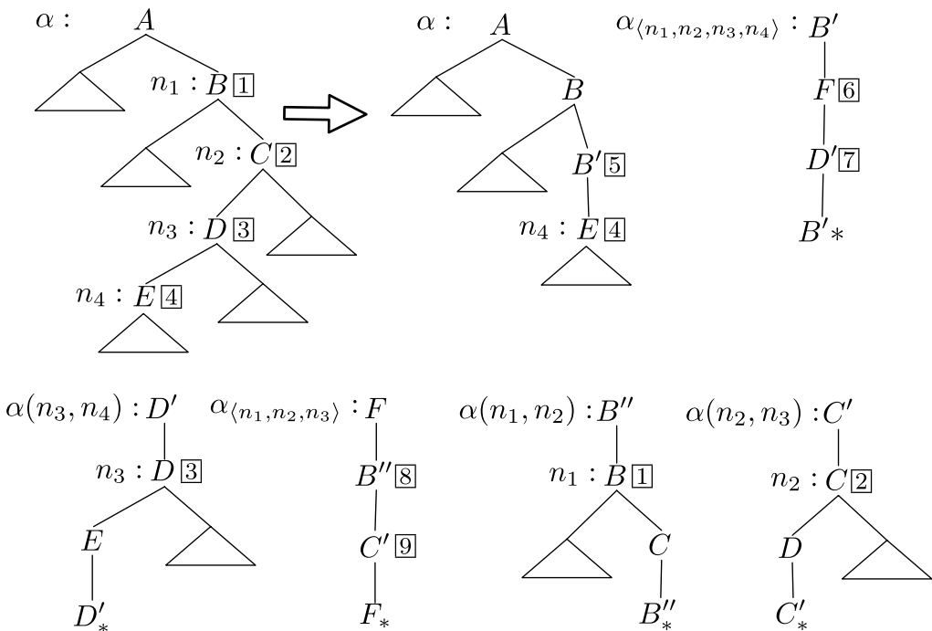
Figure 17 The binarization procedure applied to a maximal chain c = \langle n_1, n_2, n_3, n_4 \rangle .
