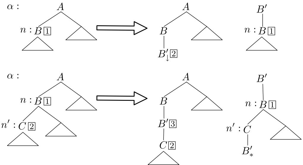
Figure 16 Diagrams of the tree transformations performed when fragments \alpha(n) and \alpha(n, n') are removed.
