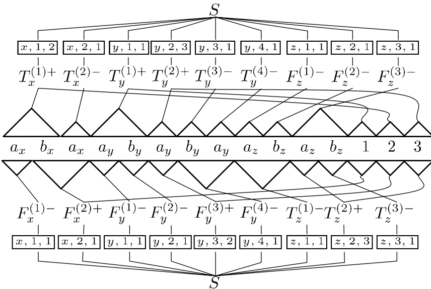
Figure 5 Example derivations of two satisfying assignments for the boolean formula (\bar{x} \vee y \vee z) \wedge (x \vee \bar{y} \vee \bar{z}) \wedge (y \vee \bar{y} \vee z) .
