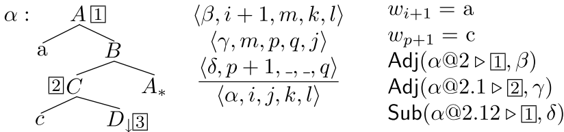
Figure 7 The deductive rule generated for tree \alpha using the naive TAG parsing method.
