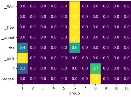
(a) Latent Grouping
