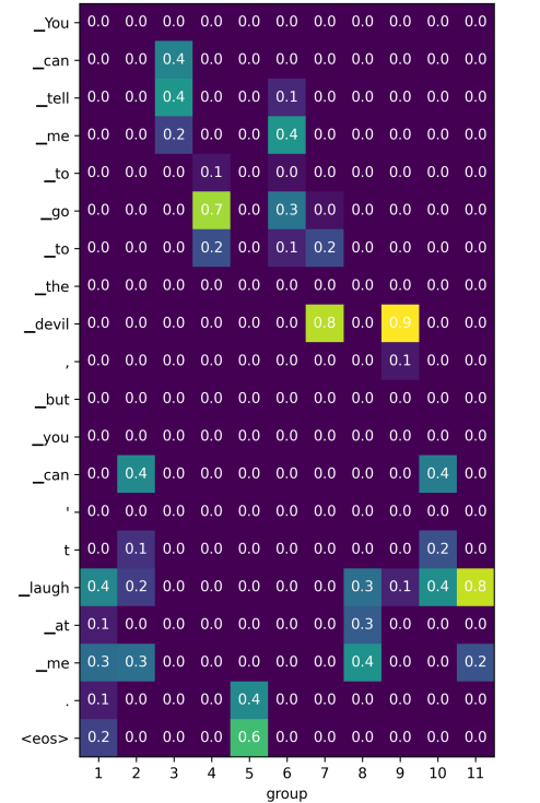
(f) Latent Selecting
