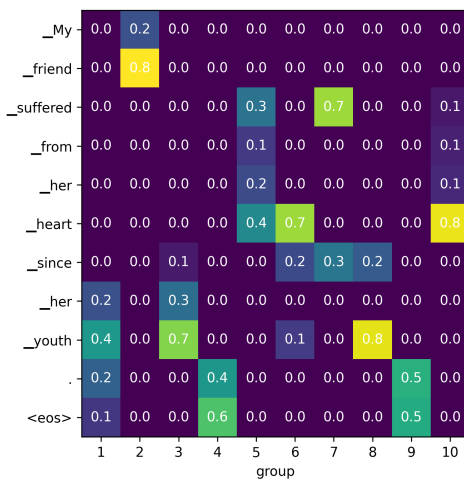
(b) Latent Selecting
