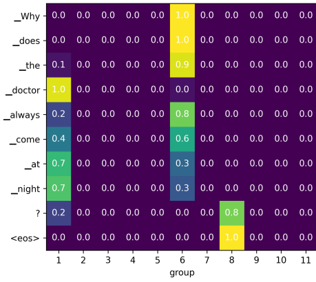
(c) Latent Grouping
