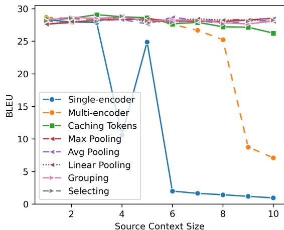
Figure 3: BLEU of the models trained on the En-De IWSLT 2017 dataset with the context sizes up to 10. Caching Sentence model was not included for clarity.
