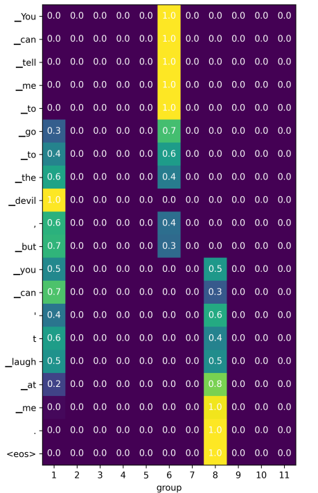
(e) Latent Grouping
