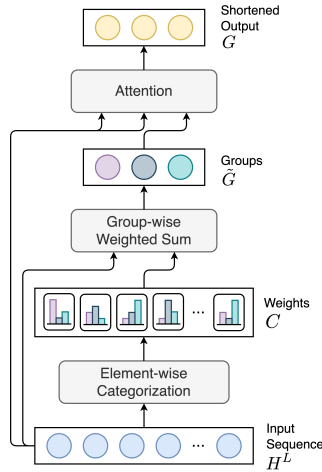
Figure 1: Illustration of Latent Grouping shortening with the number of groups set to three.
