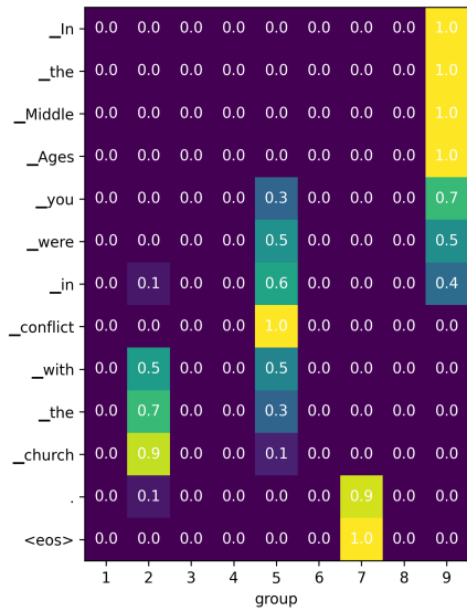
(c) Latent Grouping
