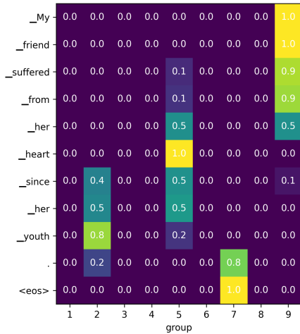
(a) Latent Grouping
