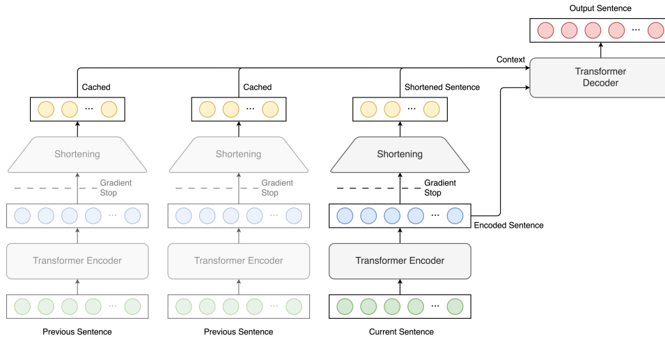
Figure 2: The illustration of a Shortening Architecture with the representation of the two previous sentences being cached. The dashed line represents the optional blocking of the gradient during training.
