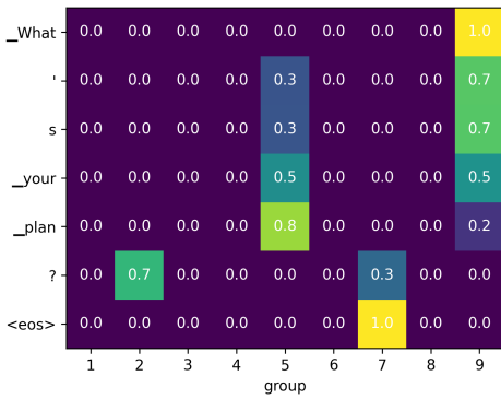
(a) Latent Grouping
