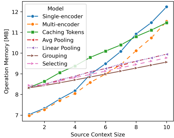
Figure 5: The mean operation memory of the models when performing inference on the examples from the En-De IWSLT 2017 test subset with the varying context sizes. For the context sizes above three, we used the models trained on the context size of three.
