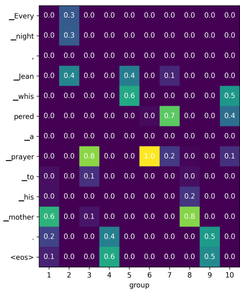
(f) Latent Selecting
