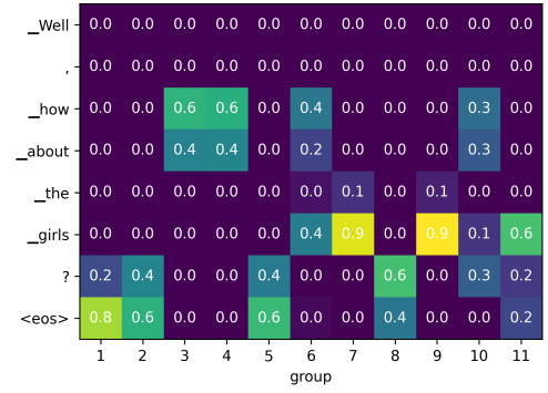
(b) Latent Selecting
