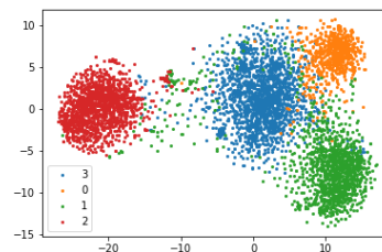
Figure 1: TSNE of speaker embeddings from a speaker encoder. The labels are obtained by applying k -means clustering with k = 4 .
