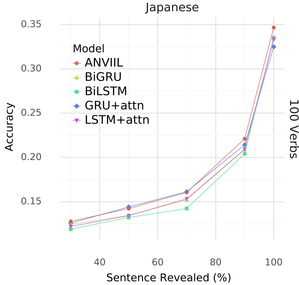
Figure 6: ANVIII’s BiGRU with self-attention outperforms other most settings on predicting the 100 most common verbs in Japanese.
