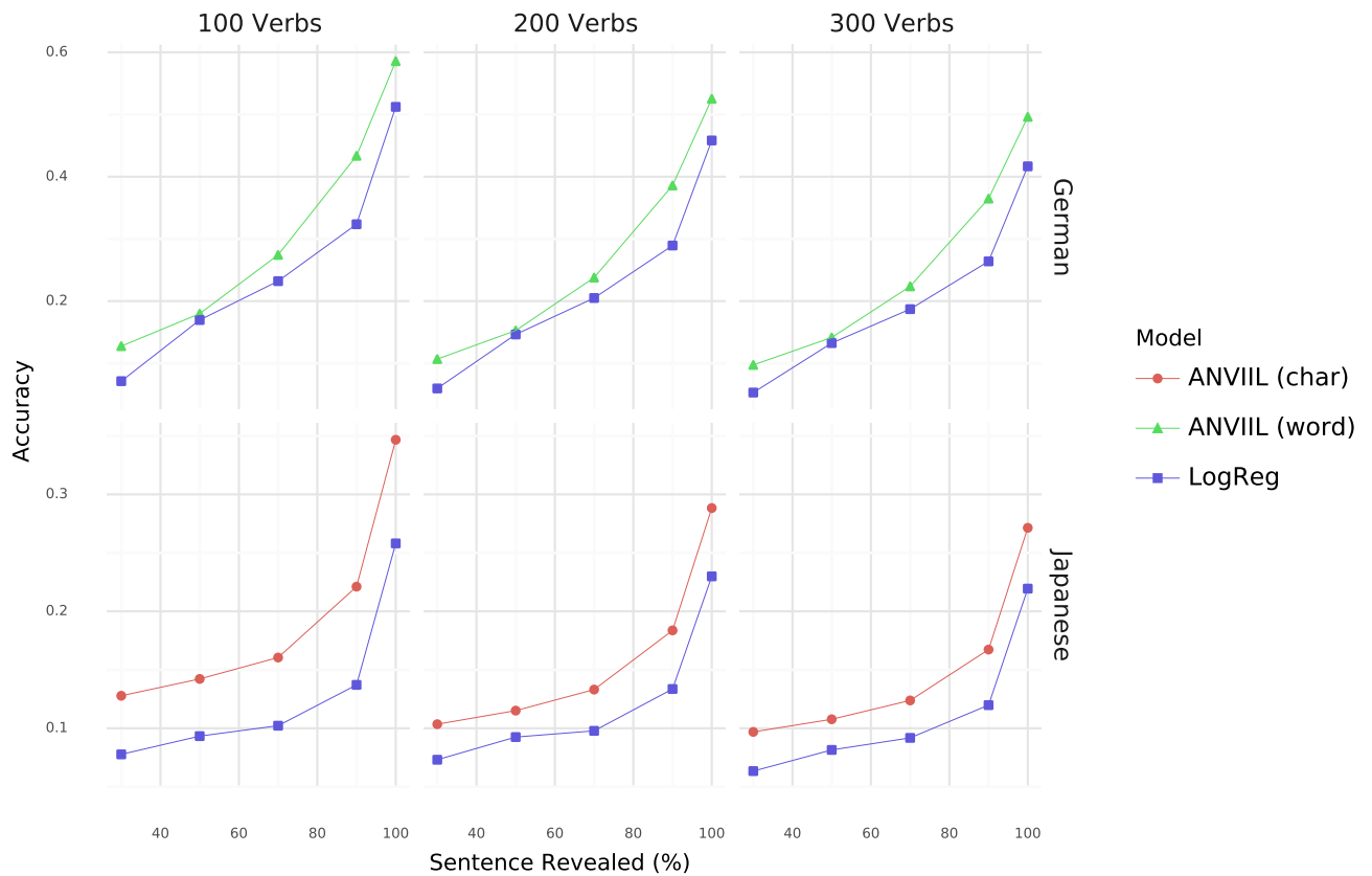
Figure 5: Accuracy when classifying among the most common 100, 200, and 300 verbs. ANVIIL consistently outperforms the best-performing model described in Grissom II et al. (2016), especially early in the sentences.
