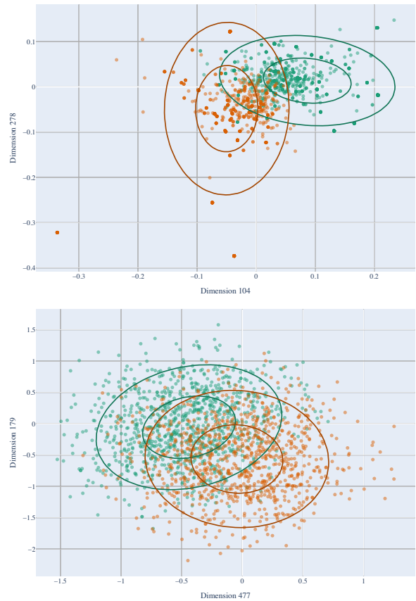
Figure 5: Scatter graph of two most informative fastText (above) and BERT (below) dimensions for English present and past tense. Contours belong to our probe.
