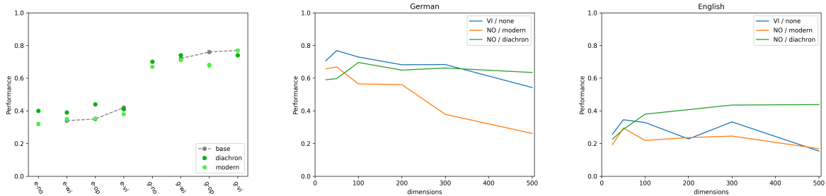
Figure 2: Left: max scores from Table 2, middle and right: Performance (Spearman’s rho) of NO alignment method on LCS D task across different dimensionalities and pre-training corpora. VI without pre-training as comparable baseline.
