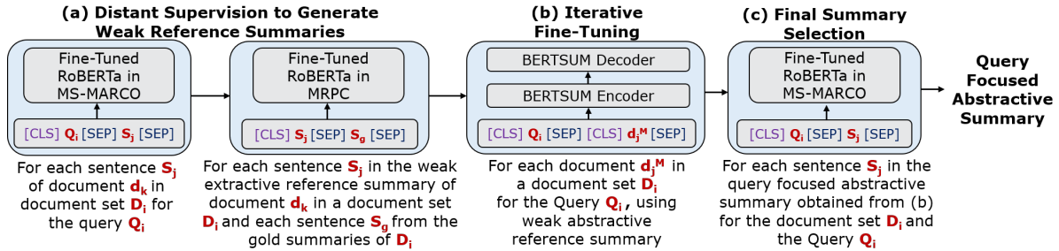
Figure 1: An overview of our model that generates (a) weak reference summary using RoBERTa for (b) iterative fine-tuning using BERTSUM to generate query focused abstractive summaries which are then ranked by (c) RoBERTa . [CLS] and [SEP] are the special tokens used with inputs (Devlin et al., 2019).
