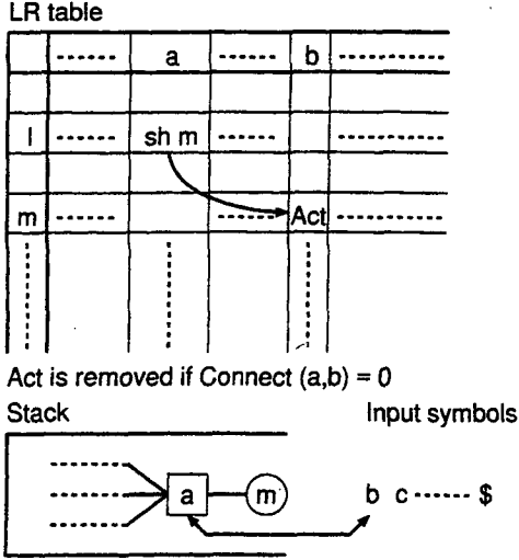
Figure 3: LR table and Connection Constraints
