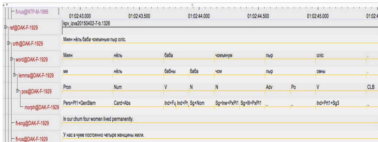
Figure 2: The result of the last processing step – (partial) disambiguation of morphosyntactic ambiguous analyses for the same Komi sentence as in Figure 1: for instance, for the word form чомъянум the contextually appropriate noun reading with lemma чом is chosen while the adjective reading with lemma чомъя is discarded.
