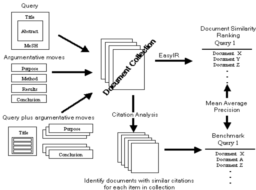
Figure 2: Flowchart for the chain of experimental procedures. The benchmark was assembled from citations shared between documents and compared to the document similarity ranking of EasyIR.
