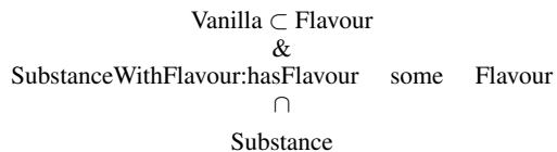
Figure 1: Complex subclass example in OWL
