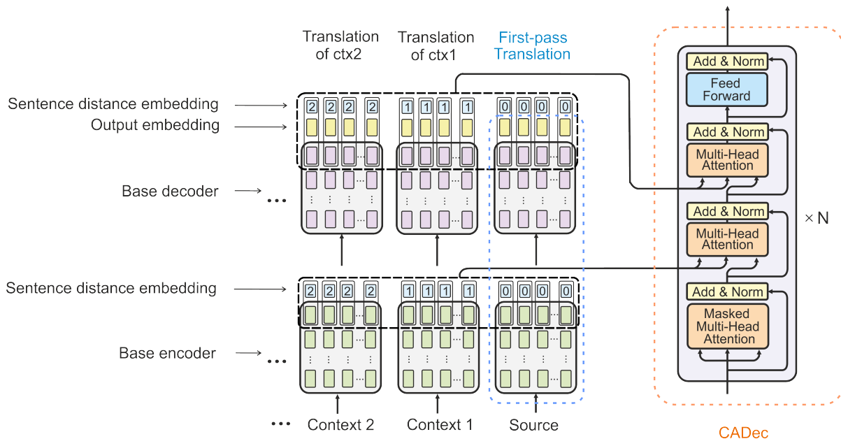
Figure 4: Model architecture
