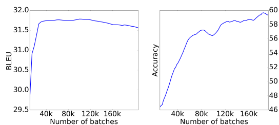
Figure 5: BLEU and lexical cohesion accuracy on the development sets during CADec training.
