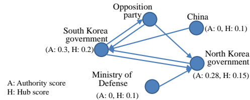
Figure 1. Example HITS graph illustration
