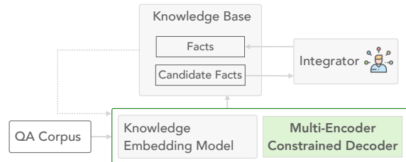
Figure 4: Human-in-the-loop system for extending a domain-specific KB.
