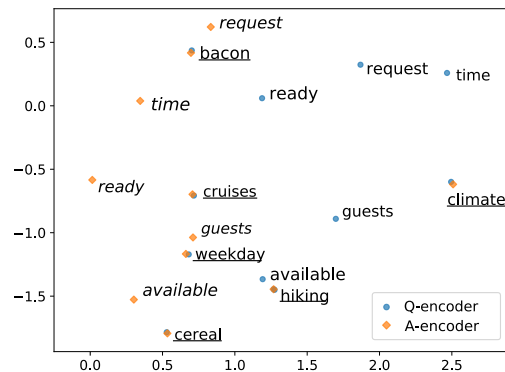
Figure 3: Example embedding vectors from question and answer encoders. Underlines denote similar embedding vectors in both the encoders.
