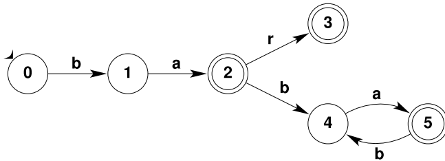
Figure 4 Minimal automaton accepting the set of strings (ba)^+ \cup \{\bar{b}\} .
