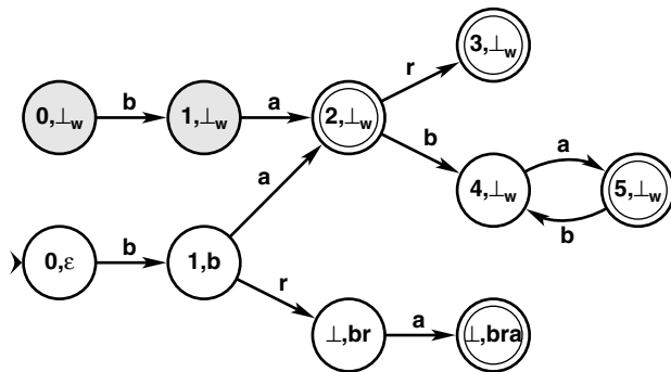
Figure 6 Unminimized automaton accepting the set (ba)^+ \cup \{\bar{b}\} \cup \{\text{bra}\} . Shaded states (0, \perp_w) and (1, \perp_w) have become unreachable (have no incoming transitions) and are eliminated in precisely that order.
