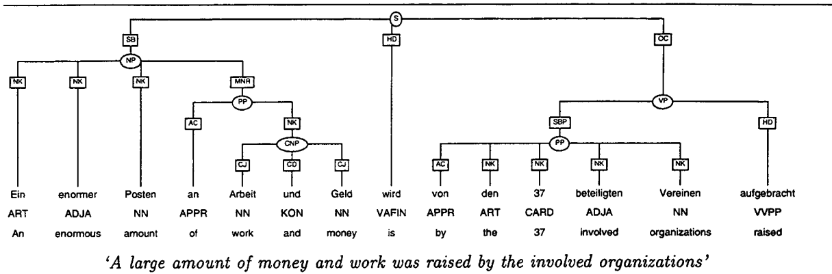
Figure 1: Example sentence and annotation. The structure consists of terminal nodes (words and their parts-of-speech), non-terminal nodes (phrases) and edges (labeled with grammatical functions).
