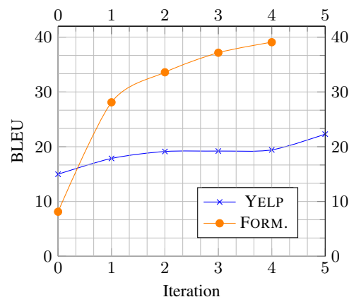
Figure 2: BLEU score evolution across training iterations on YELP and FORMALITY datasets.
