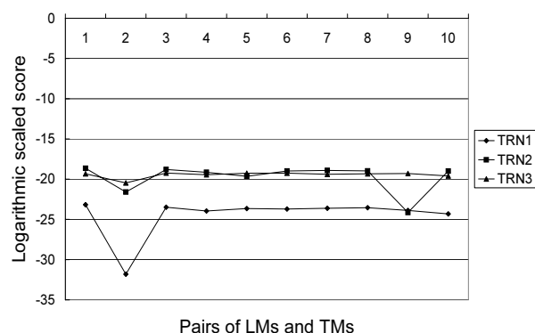
Figure 4: The same translation can be scored differently by TM*LM-score.
