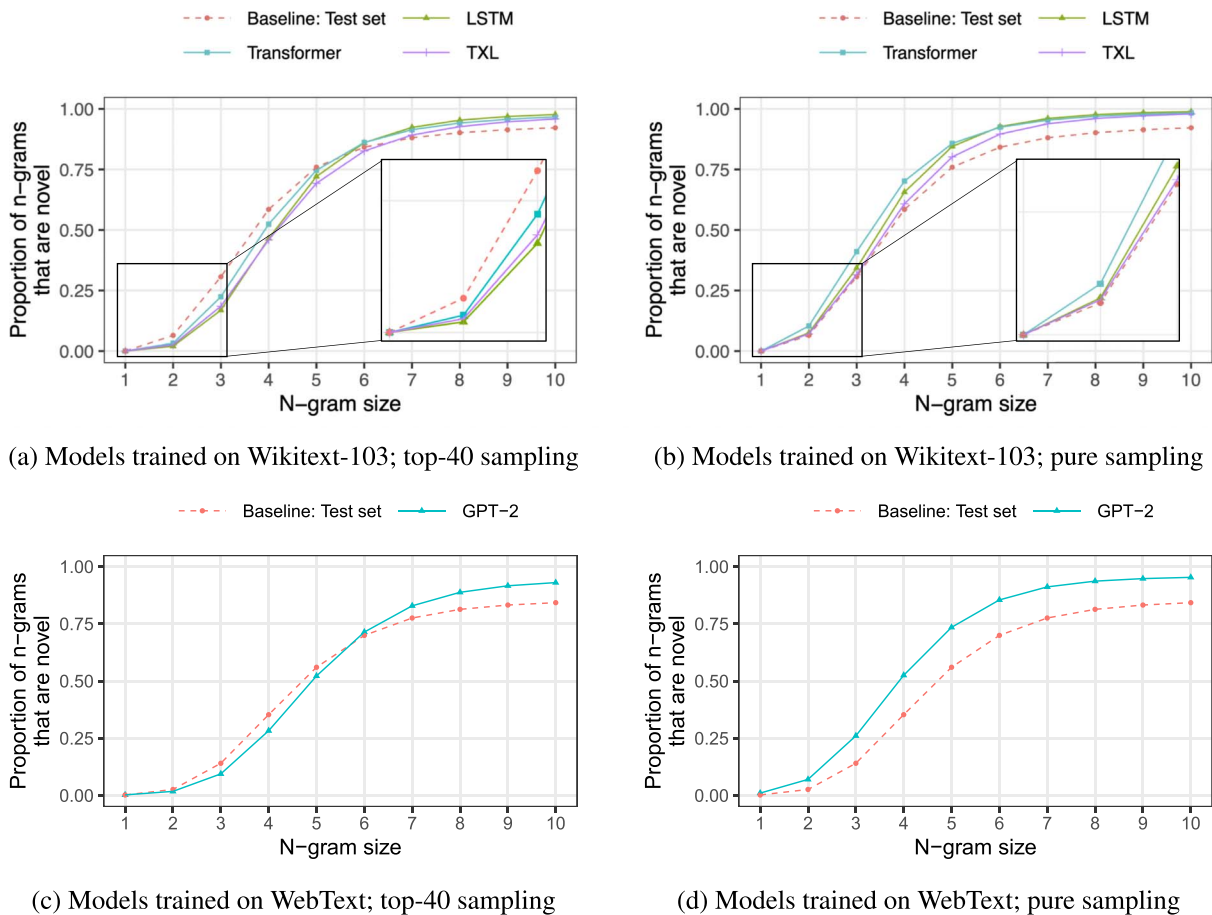
Figure 1: Novelty of n -grams generated by LMs using top-40 sampling (which is the approach used in relevant prior literature) and pure sampling (which uses a model’s unaltered distribution but is not standard because it produces low-quality text). As baselines, we use text drawn from models’ test sets.
