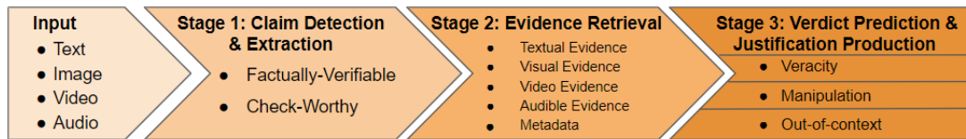
Figure 2: Multimodal fact-checking pipeline.
