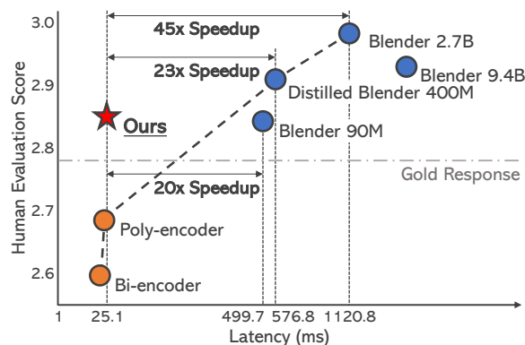
Figure 1: Latency vs. Human evaluation score plot for open-domain conversation models. Blue circle represents generative models, orange circle represents retrieval models, and red star represents our model. Our model achieves a "sweet-spot" among various models, showing a much better human evaluation score than retrieval models and demonstrating much lower latency than generative models.
