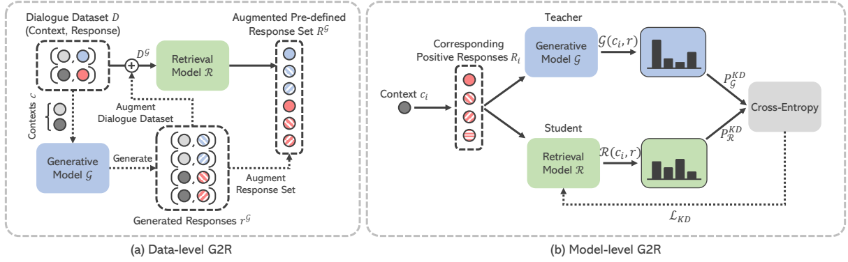
Figure 2: Illustration of our proposed training method G2R.
