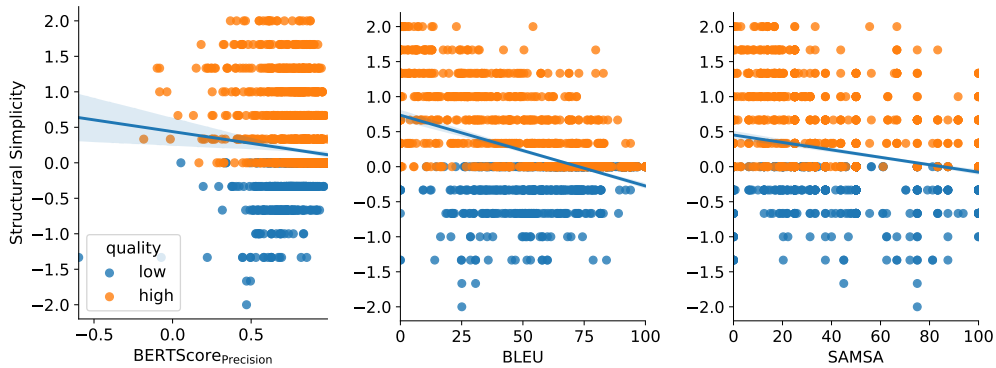
Figure 6 Scatter plots showing the correlation ( r ) between \text{BERTScore}_{\text{Precision}} , BLEU, and SAMSA, with human rating of Structural Simplicity, for different quality levels.
