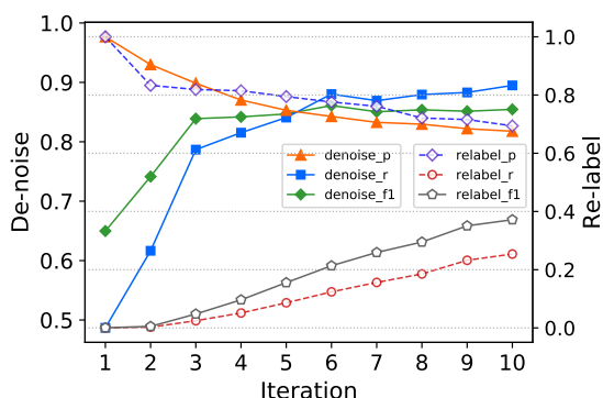
Figure 4: Data-refining details on noisy-TACRED.
