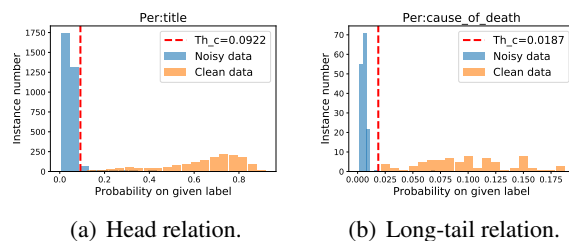
Figure 5: Data distribution of a head relation (per:title) and a long-tail relation (per:cause_of_death) during NT. The dynamically designed thresholds benefits filtering.
