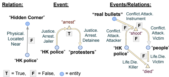
Figure 2: In the case of events, we ignore the event trigger denoted by \triangle and connect entities by their event argument roles and event types combined e.g., \langle HK\ police, Justice.Arrest.Jailer-Justice.Arrest.Detainee, (un-cooperative)\ protesters \rangle . The True/False tags are labeled for each triplet, which connects a pair of entities.
