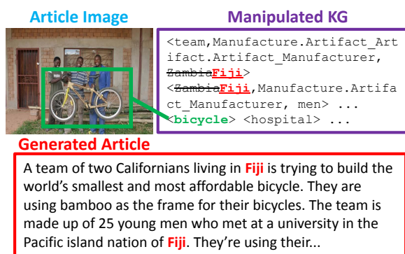
Figure 3: We show example of manipulating the multimedia KG of a news article, swapping geolocation-typed entity “Zambia” with “Fiji”.
