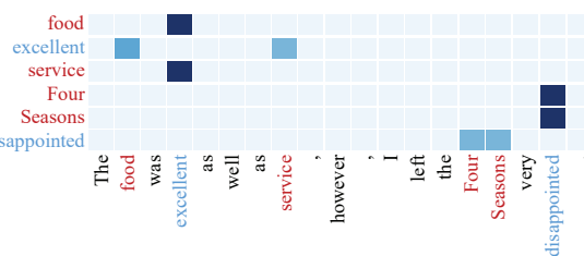
Figure 4: Visualization of attention scores. The aspects and the opinion expressions are marked with red and blue, respectively. (Best viewed in color.)
