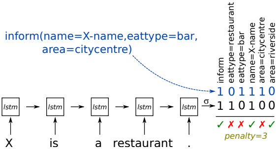
Figure 4: The reranker
