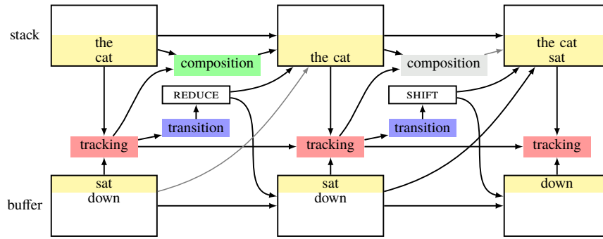
(a) The SPINN model unrolled for two transitions during the processing of the sentence the cat sat down . ‘Tracking’, ‘transition’, and ‘composition’ are neural network layers. Gray arrows indicate connections which are blocked by a gating function.
