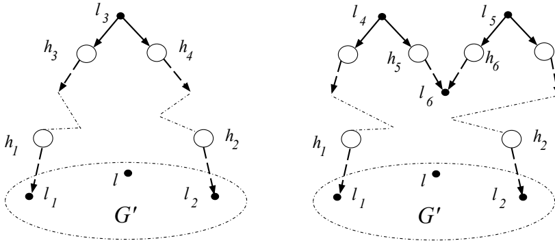
Figure 19 Proof of Lemma 10.
