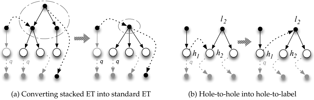
Figure 6 Conversion to original UG.
