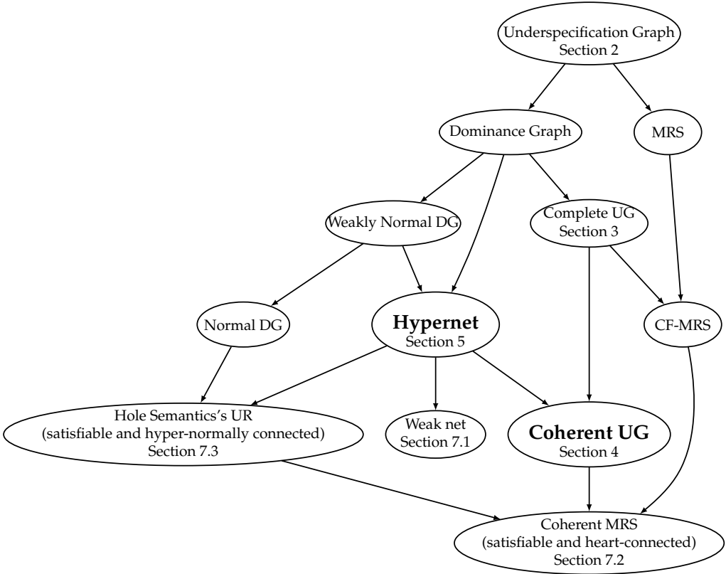
Figure 1 Classes of underspecification graph introduced in this article. We define hypernet, show that it is computationally tractable, and further show that it covers all coherent sentences, and that it subsumes previously identified tractable classes.
