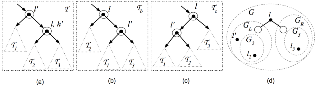
Figure 15 Proof of Theorem 9.
