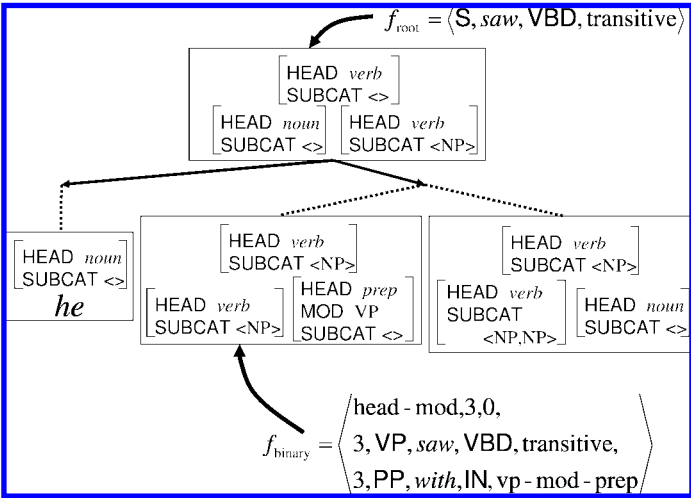
Figure 20 Example features for binary schema application and root condition.
