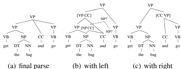
Figure 1: Parsing with left and right binarization.
