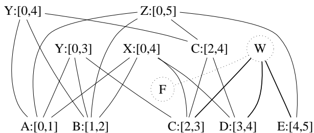
Figure 2: Parse of the sentence ABCDE
