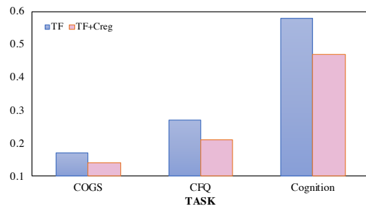
Figure 4: Intra-class variance of Transformer (TF) and regularized Transformer (TF+CReg) on CFQ and CoGnition.
