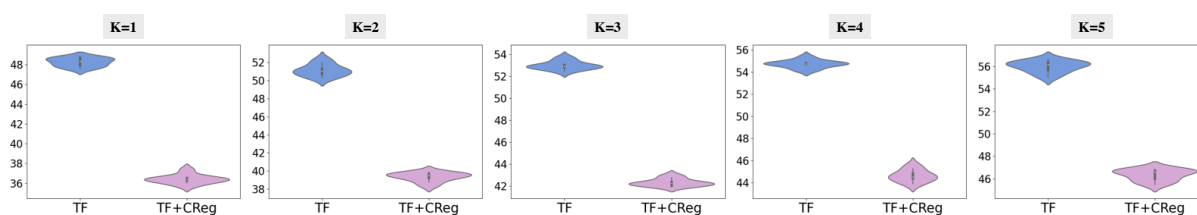
Figure 6: Effect of input noise on CoGnition. K represents the number of tokens that are replaced at random in the context part of a source sentence. The vertical axis represents the average of instance and aggregate CTER.
