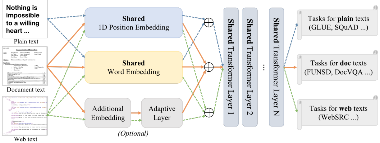
Figure 3: XDoc tackles multiple formats in one model while sharing most parameters including 1D position embedding, word embedding, and dense Transformer layers. An optional embedding layer and adaptive layer are utilized for specific prior knowledge such as 2D position for document texts and XPath for web texts (no additional prior for plain texts). We demonstrate the dataflow for document texts and use dash lines for other formats.
