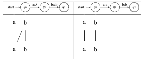
Figure 1: Pair of 1-way FSTs for the function f_{ab} and their origin information for the mapping ab \rightarrow ab .
